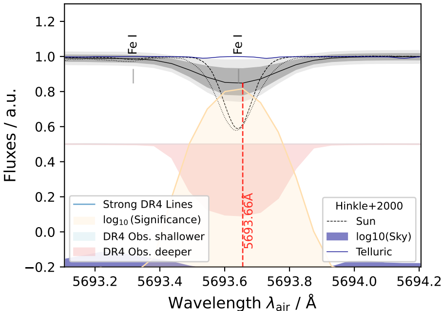
GALAH DR4 Residual at \lambda_{\text{air}} = 5693.66\text{\AA}
