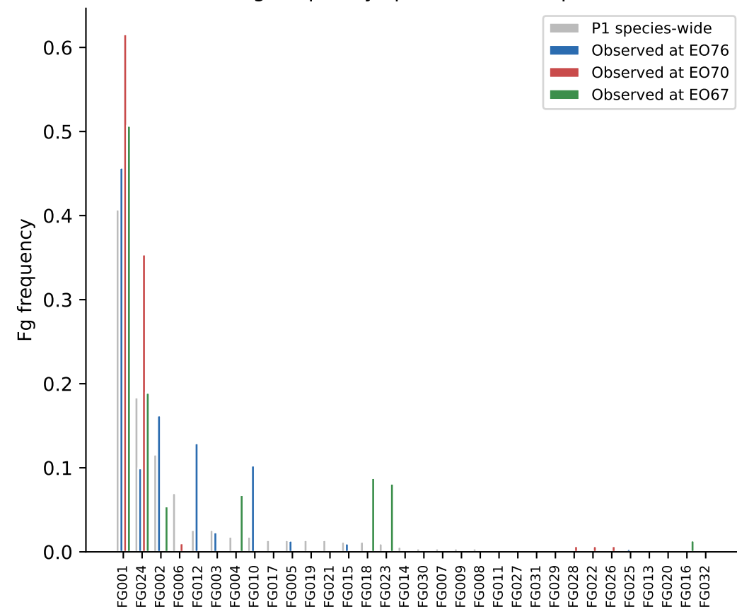
C — Observed Fg frequency spectrum vs P1 species-wide
