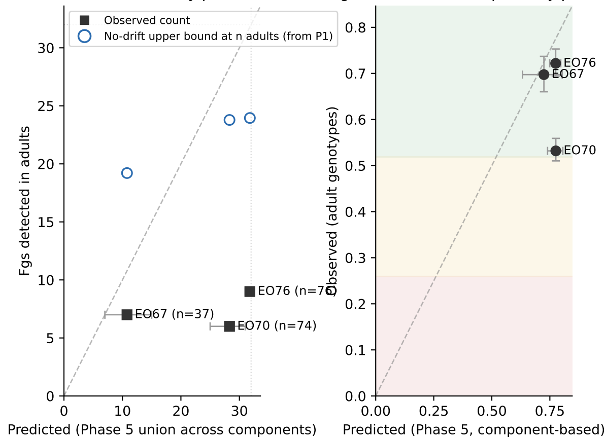
A — SRK diversity per location (ceiling = 32) — Pollen compatibility per location
