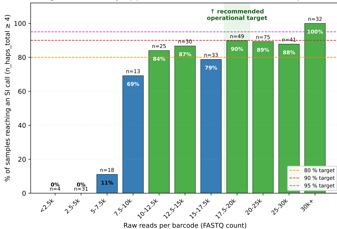
A. Dose-response — pass rate vs raw read budget (coverage-driven cohort only — pipeline-failure / chimera / DNA-contamination samples excluded)
