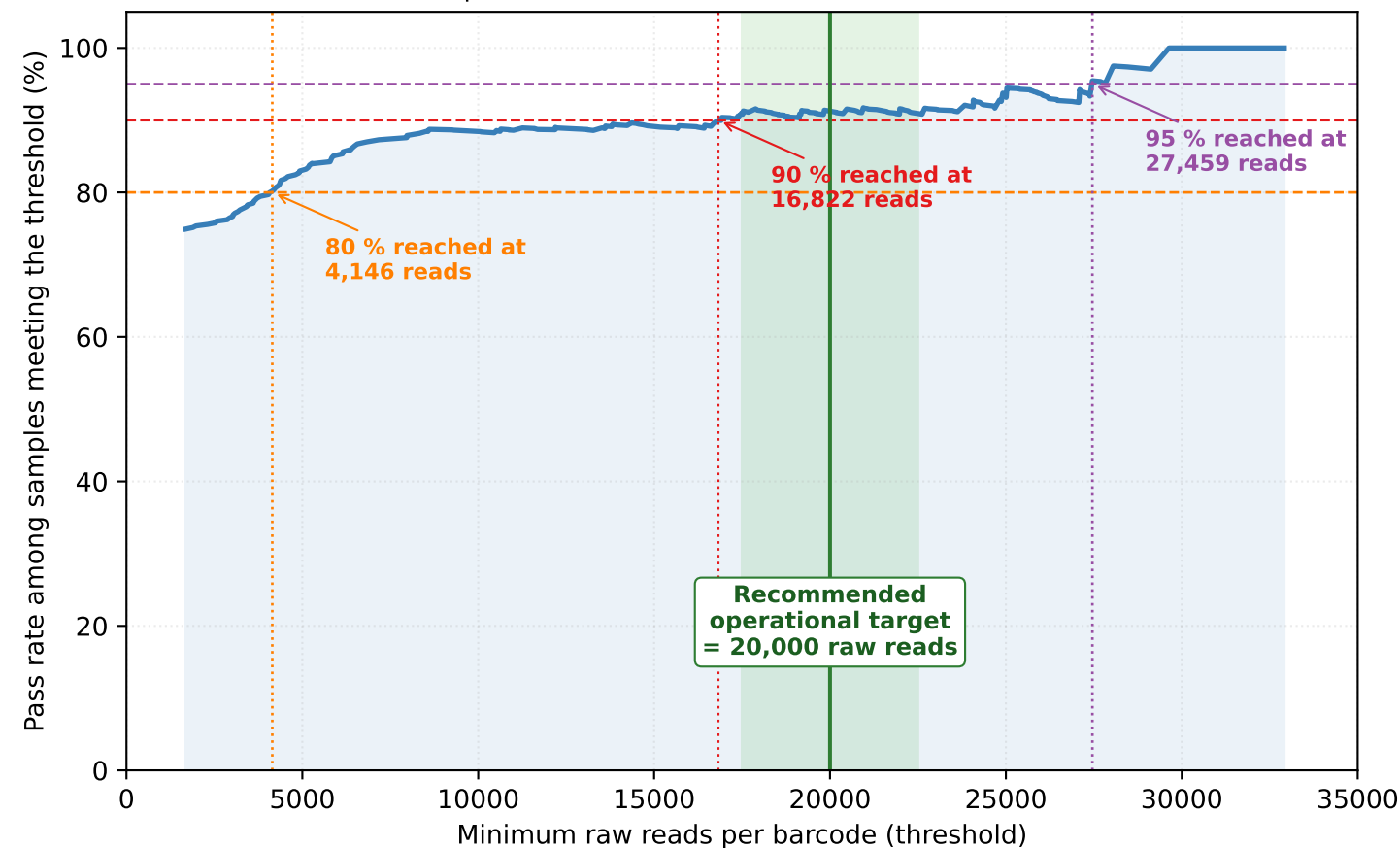
B. Cumulative pass rate — choose a threshold, read off the success rate
