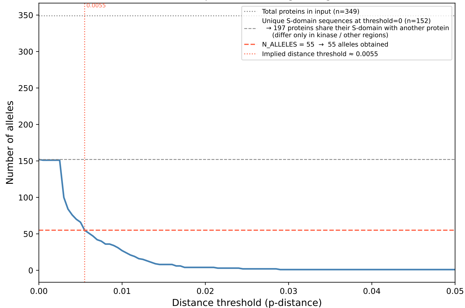
Sensitivity: allele count vs. clustering threshold (S-domain p-distance, average linkage)
