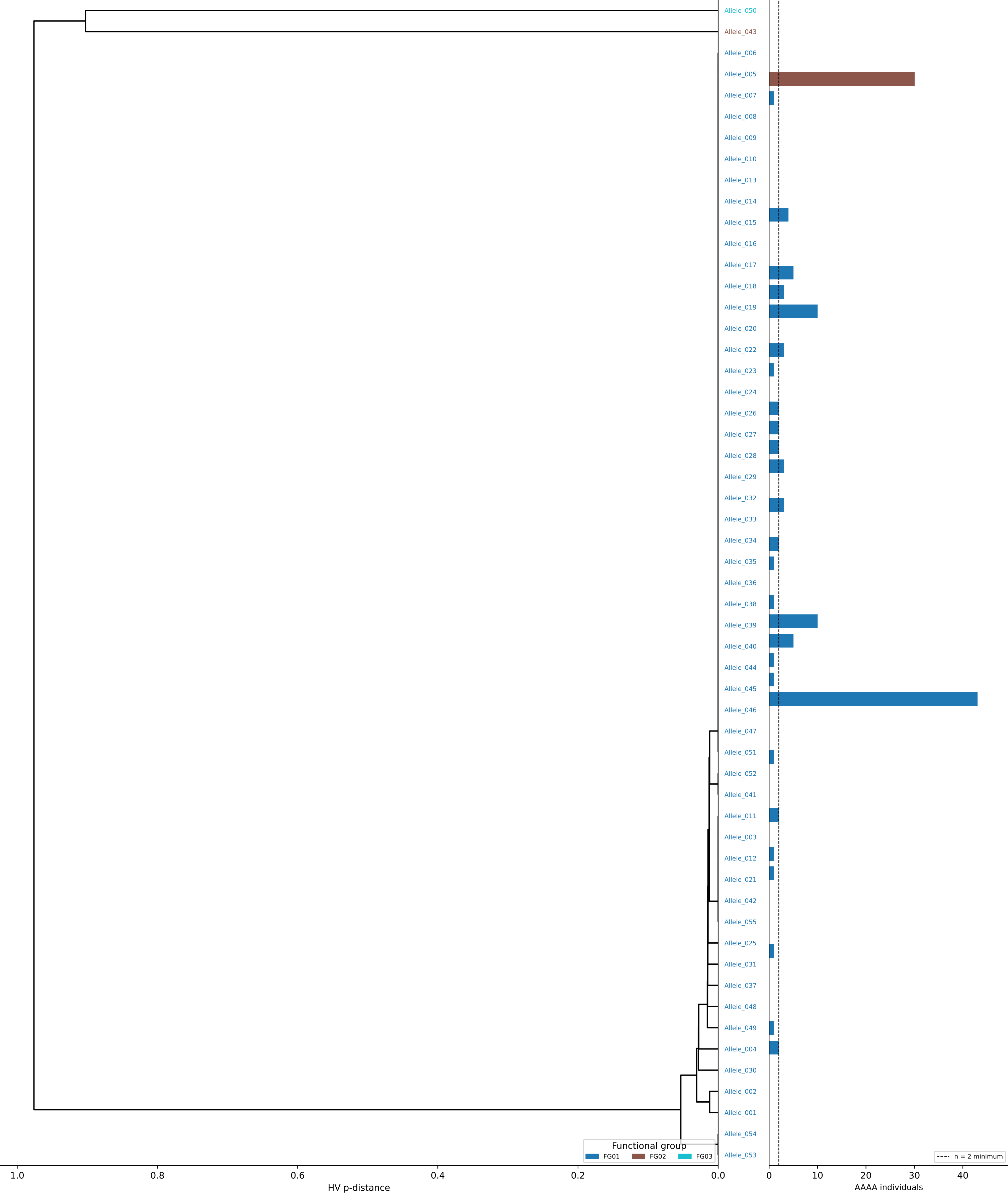
Allele functional group clustering (UPGMA, 82 HV positions, threshold = auto)
