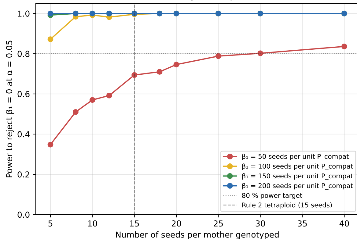
A. § C.1 mate-limitation regression power vs seed count
