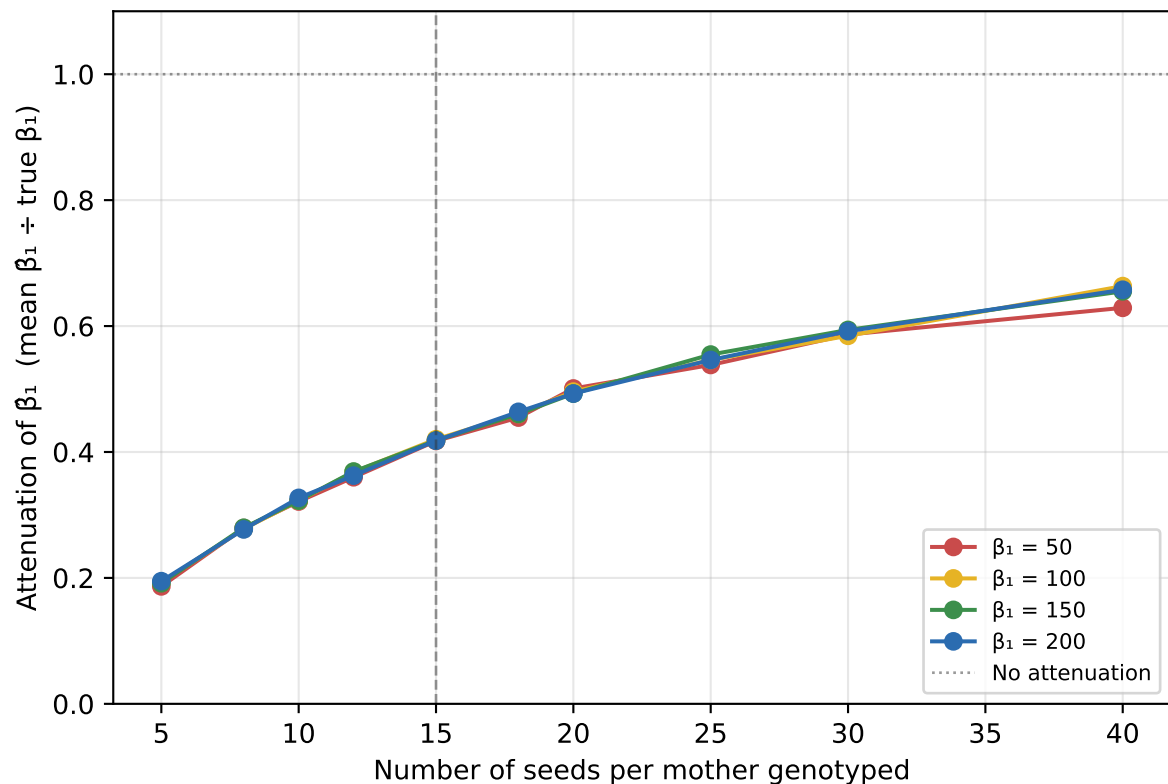
B. Errors-in-variables attenuation vs seed count
