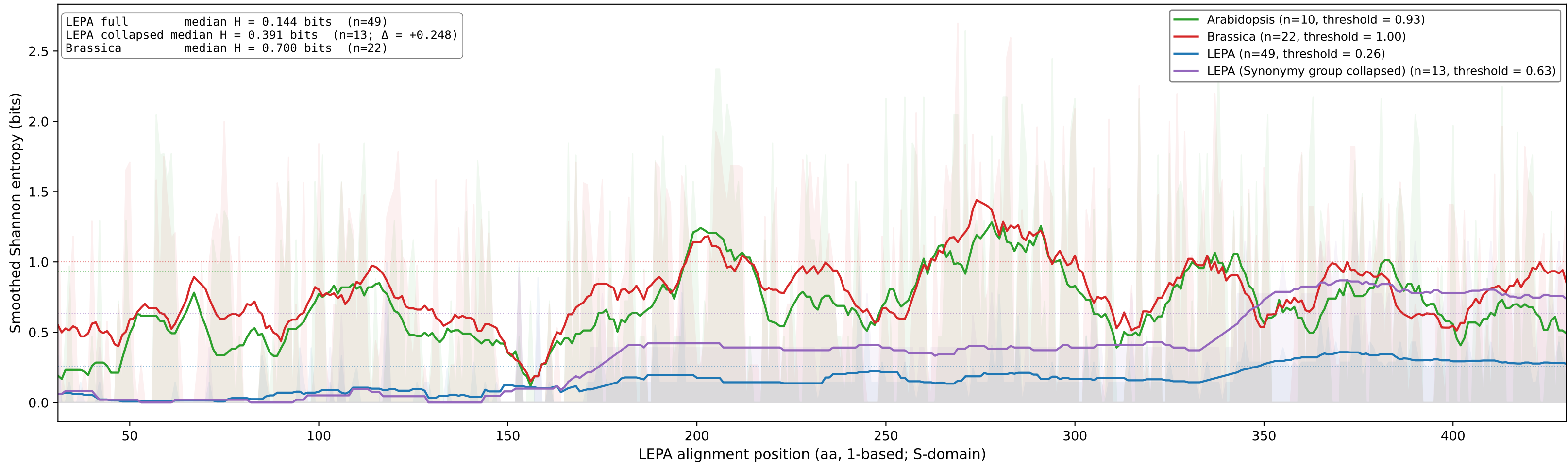
Synonymy group collapse diagnostic — does Synonymy group redundancy explain LEPA's low Shannon entropy? LEPA full (49 alleles) vs LEPA collapsed (13 Synonymy group representatives + isolated) vs Brassica vs Arabidopsis
