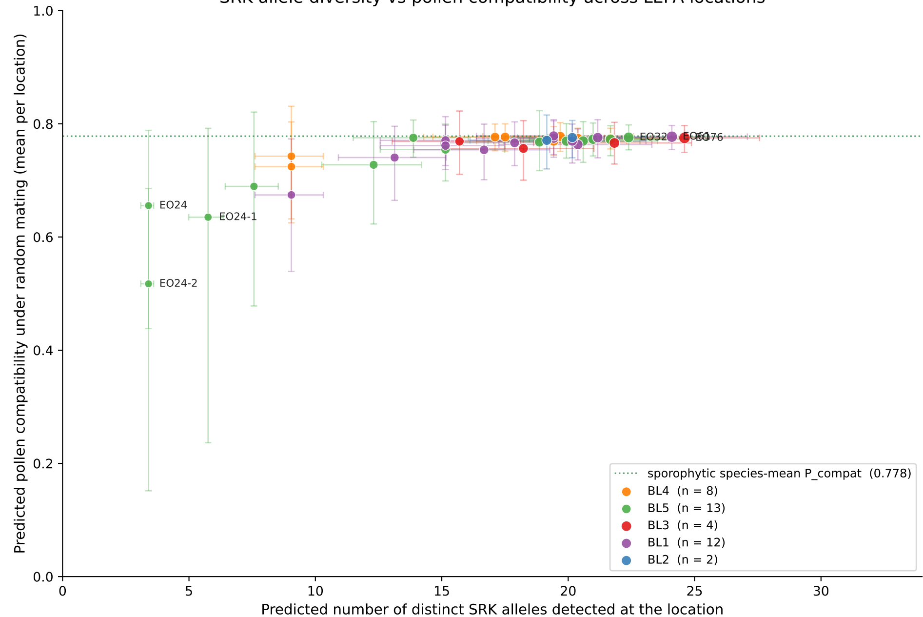
SRK allele diversity vs pollen compatibility across LEPA locations
