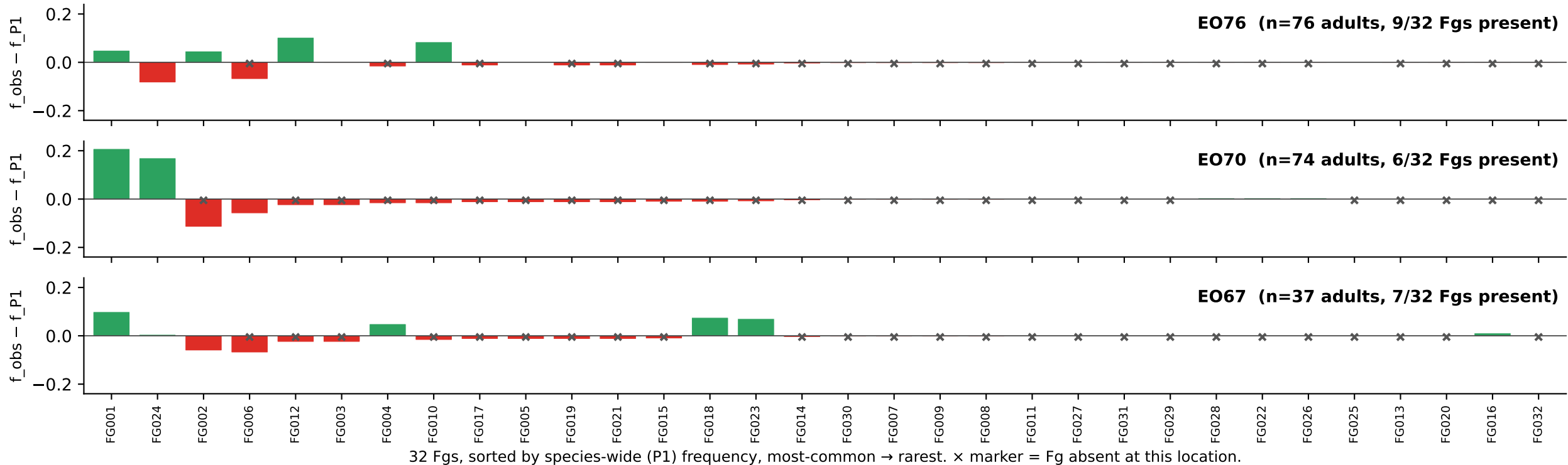
C Drift residual per Fg per location (green = observed &gt; P1; red = observed &lt; P1; x = absent)
