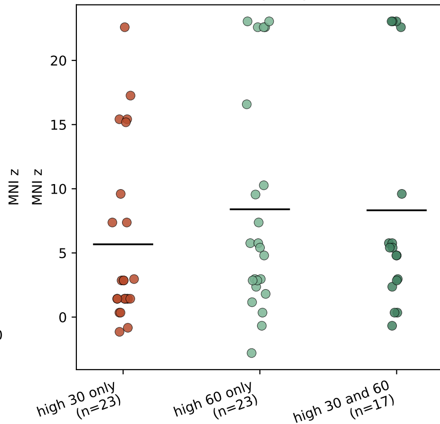
MNI z-coordinate for high-lag ACC cells
