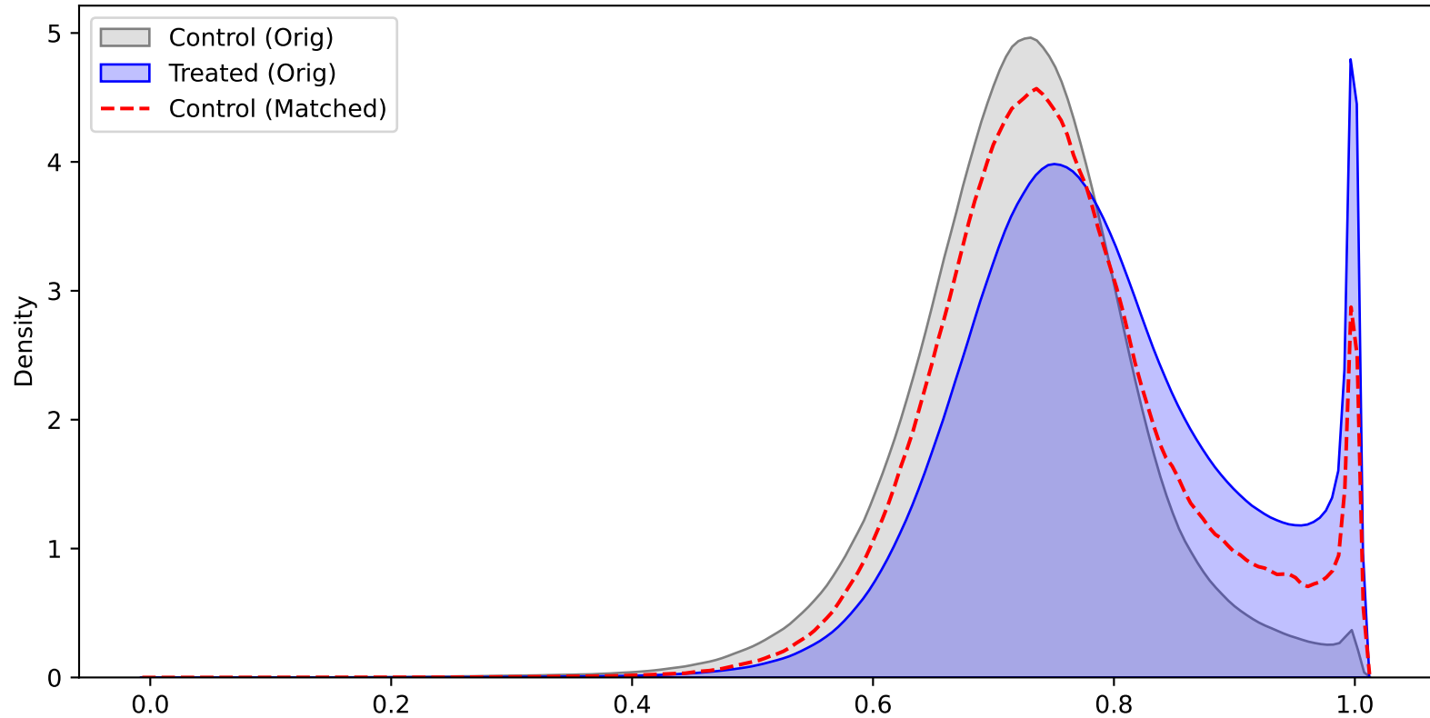
Propensity Score Support
