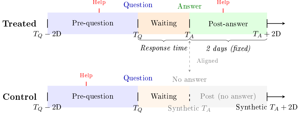
Figure 1: Study Design: Matched Difference-in-Differences Survival Analysis
