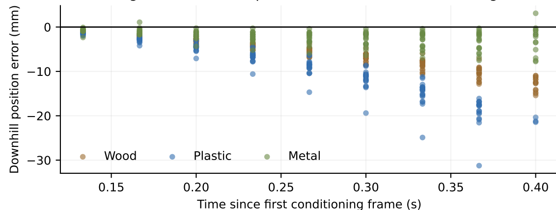
Ideal geometry rocking comparator: 134 unique first events
