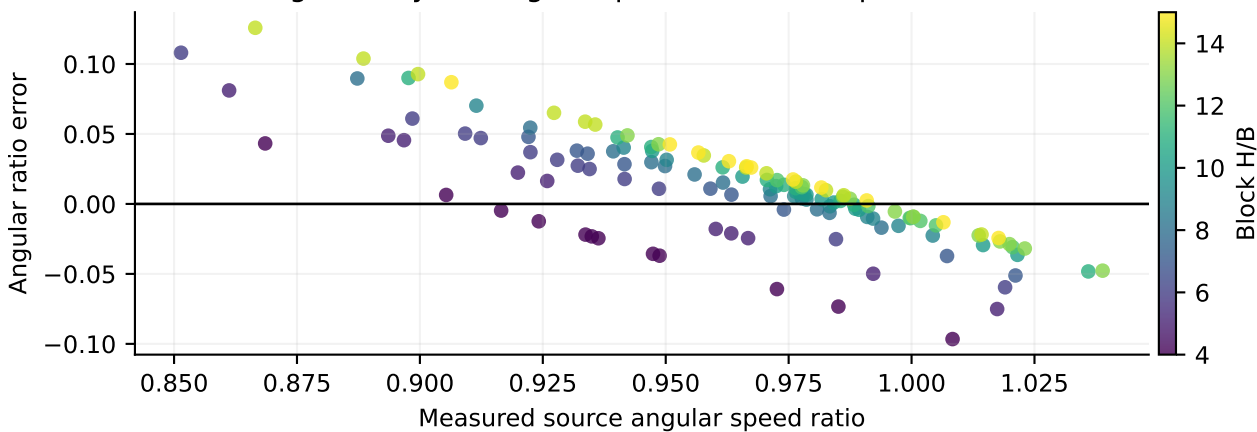
Ideal geometry rocking comparator: 134 unique first events
