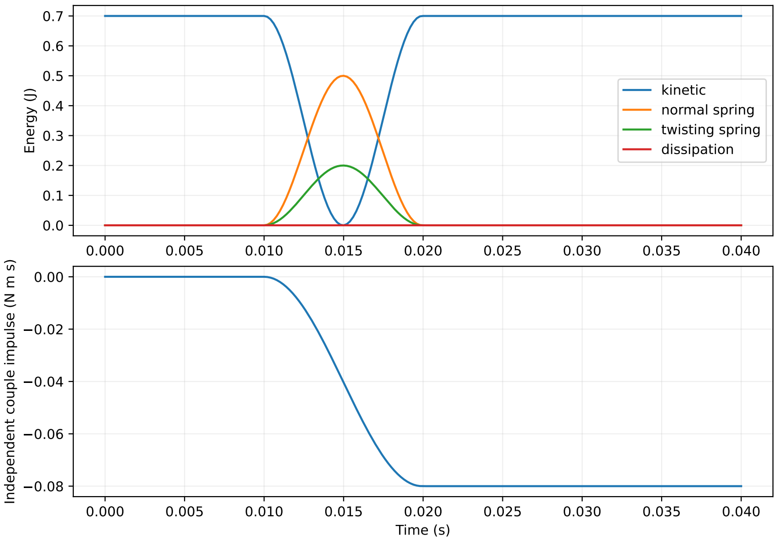
Spin reversal stores and releases torsional energy The couple impulse is separate from the moment of the point force
