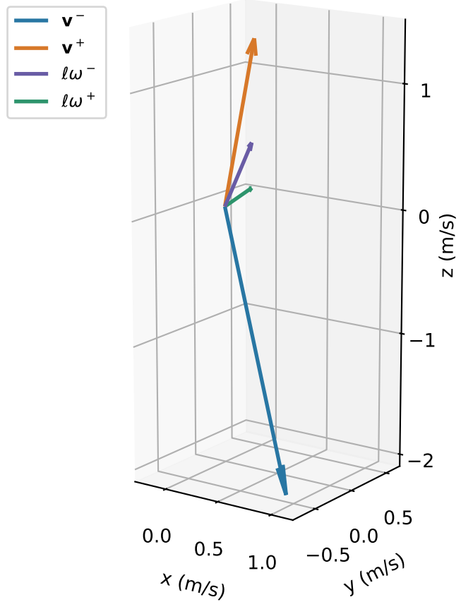
Velocity and scaled spin
