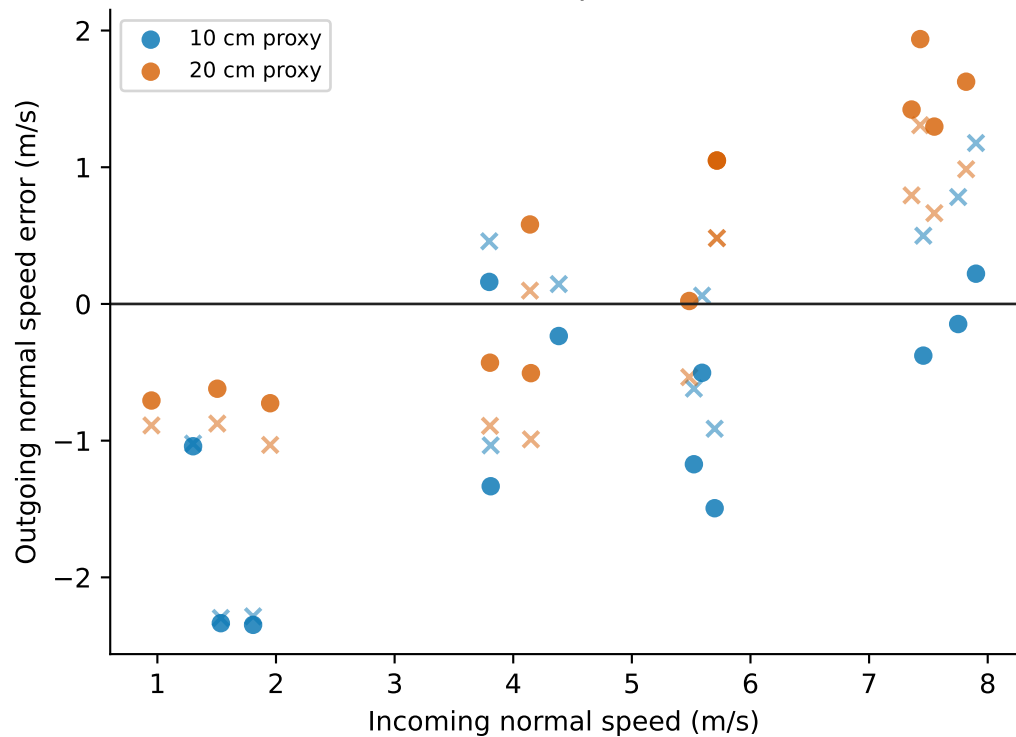
Rocks: viscoelastic sphere law is worse
