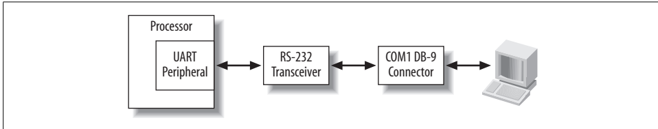
Figure 7-2. Arcom board serial port block diagram
