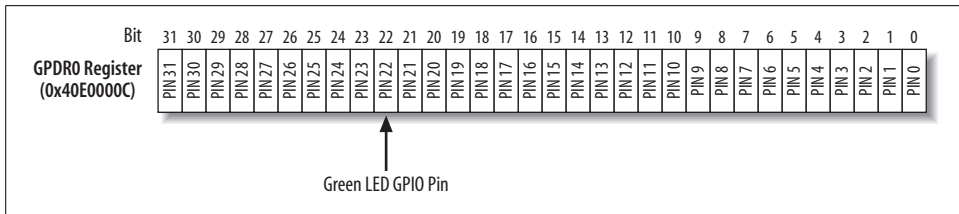
Figure 3-2. PXA255 processor GPDRO register
