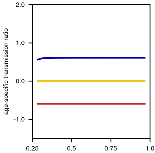
Age Specific Transmission
