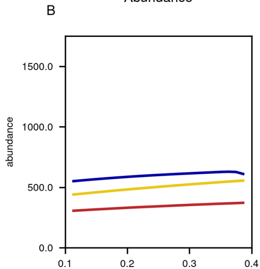
Host Abundance
