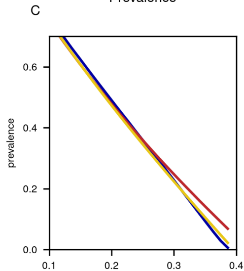
Infection Prevalence
