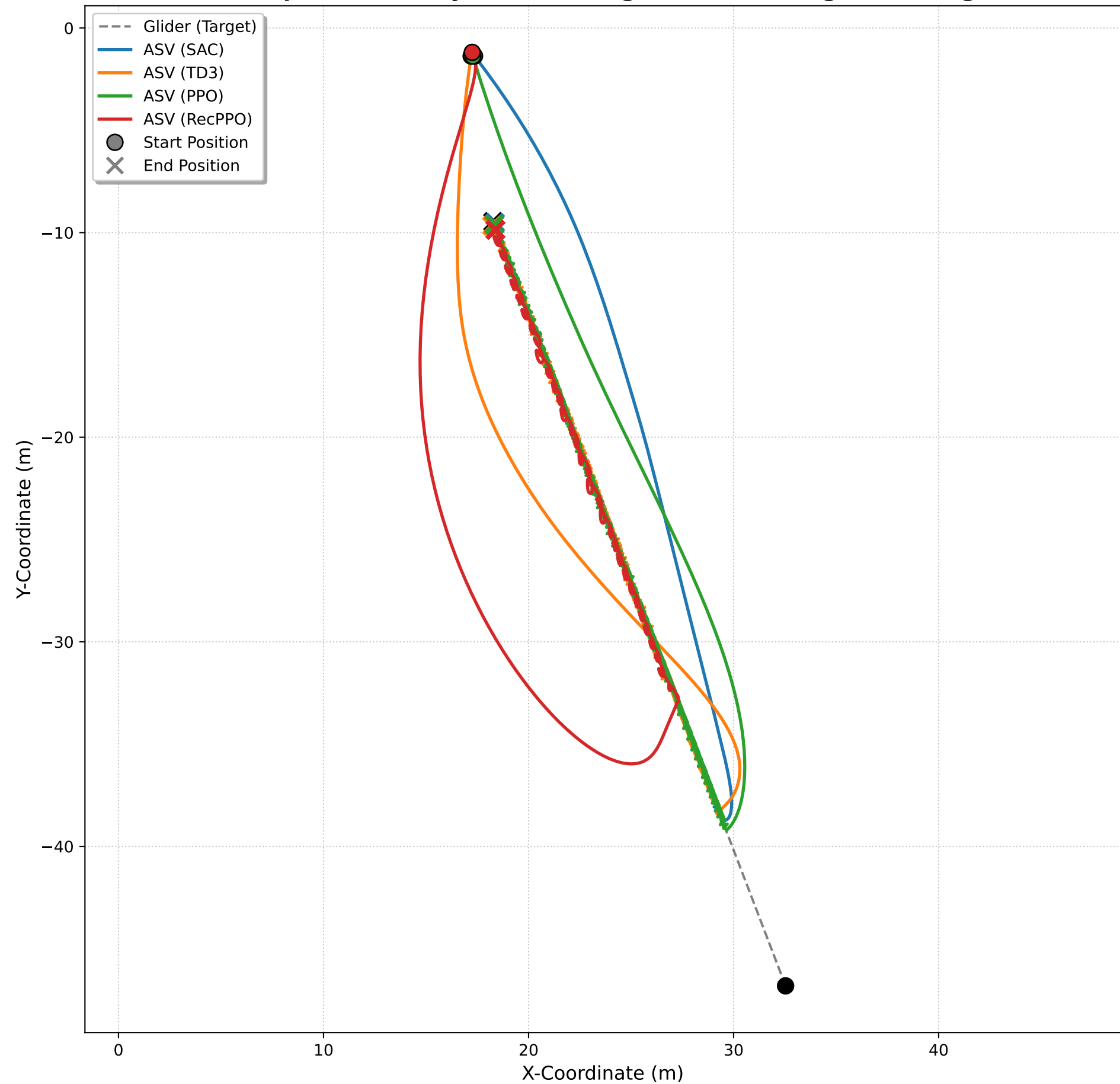
Comparative Analysis of DRL Algorithms for Target Tracking
