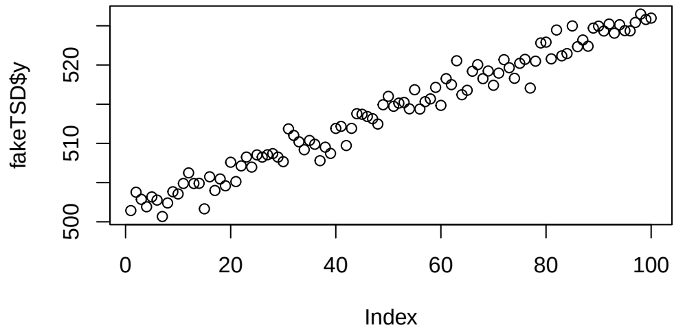
Figure A.2: A Plot of fakeTSD in {stevedata}
