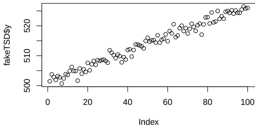
Figure A.1: A Plot of fakeTSD in {stevedata}
