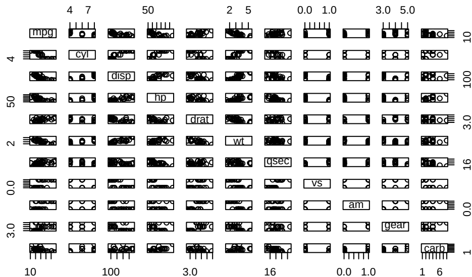
Figure A1: A Plot of the mtcars Data in Base R
