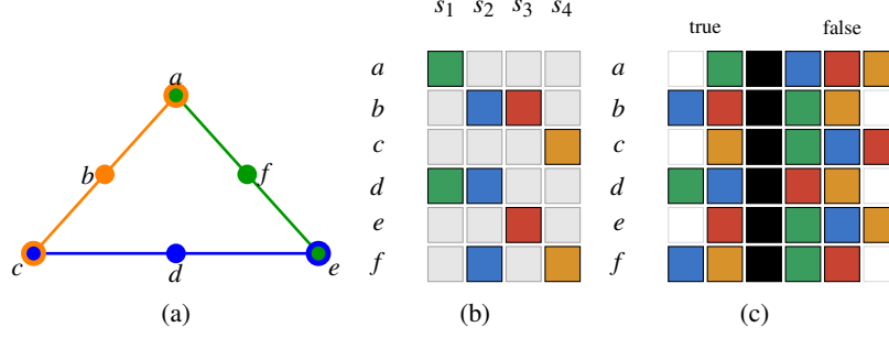
FIG. 2. Triangle-logic generalization of the Quantum Square . (a) Greechie-style depiction of the triangle logic associated with Eq. (28). The intertwining atoms a , c , and e are shown by concentric circles because each belongs to two contexts. (b) Atom-state incidence schema. (c) Tile rendering obtained from the grammar in Eq. (33), using four recurring state colors and a black separator between support and complement.
