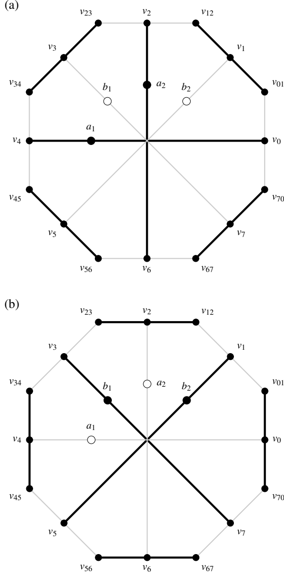
FIG. 2. Graphical representation of the two distinct coverings of the octagon hypergraph. (a) Covering A (bold lines) isolates the (a_1, a_2) pseudocontext using inner contexts D_0, D_2 and alternating outer edges. (b) Covering B (bold lines) isolates the (b_1, b_2) pseudocontext using inner contexts D_1, D_3 and the complementary outer edges. Vertices actively engaged in a covering are filled black, while the two strictly uncovered inner vertices in each panel are filled white. Since both coverings exactly partition all 16 outer vertices, their respective probability sums must equate, forcing P(a_1) + P(a_2) = P(b_1) + P(b_2) .
