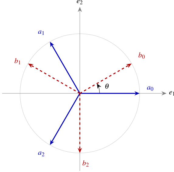
FIG. 1. The Mercedes-Benz pseudocontext of Example 23, drawn for \theta = \pi/6 . The solid blue rays a_0, a_1, a_2 and the dashed red rays b_0, b_1, b_2 are two distinct unordered triples in the plane V , yet the associated rank-one projectors have the same sum \frac{3}{2}I_V .
