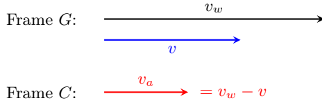
FIG. 2. Minimal kinematic definitions for Sec. IV. In the laboratory frame G , the true wind is v_w and the boat speed is v . In the vehicle frame C , the apparent-wind velocity is v_a = v_w - v . Vectors are aligned at a common origin; for v > v_w , the apparent-wind velocity v_a reverses direction.
