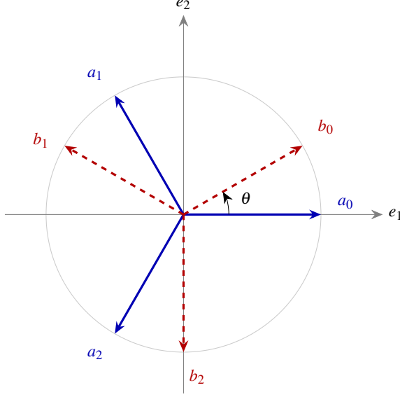
FIG. 1. The Mercedes-Benz pseudocontext of Example 17, drawn for \theta = \pi/6 . The solid blue rays a_0, a_1, a_2 and the dashed red rays b_0, b_1, b_2 are two distinct unordered triples in the plane V , yet the associated rank-one projectors have the same sum \frac{3}{2}I_V .
