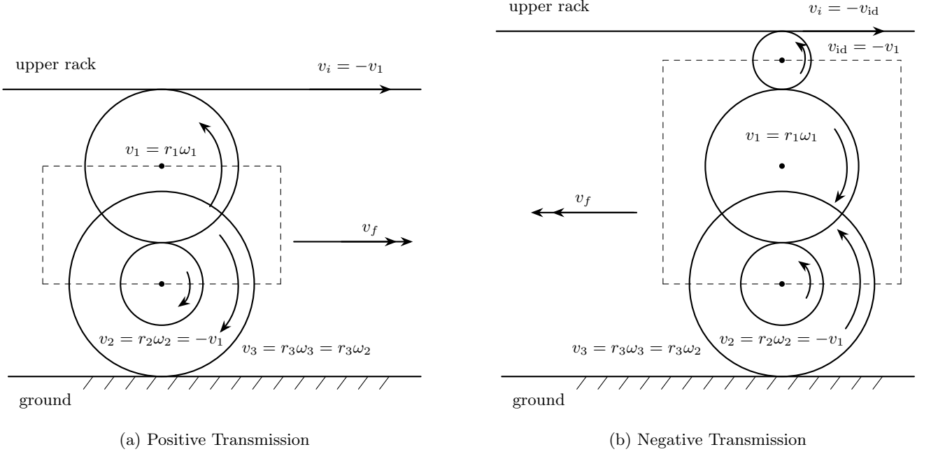
FIG. 3. Schematic of the gearbox analogy in the laboratory frame, with moving gearbox, as discussed later. Arrows indicate the direction of rotation. (a) Positive transmission (downwind): The motion of the upper rack (the wind) is transmitted through the gearbox to drive the lower rack (the ground) in the same direction, amplifying speed through the gear ratio. (b) Negative transmission (upwind): An idler gear reverses the direction of motion between the wind rack and the ground rack while preserving the same ground-constrained, no-slip coupling (traction) at the lower contact.
