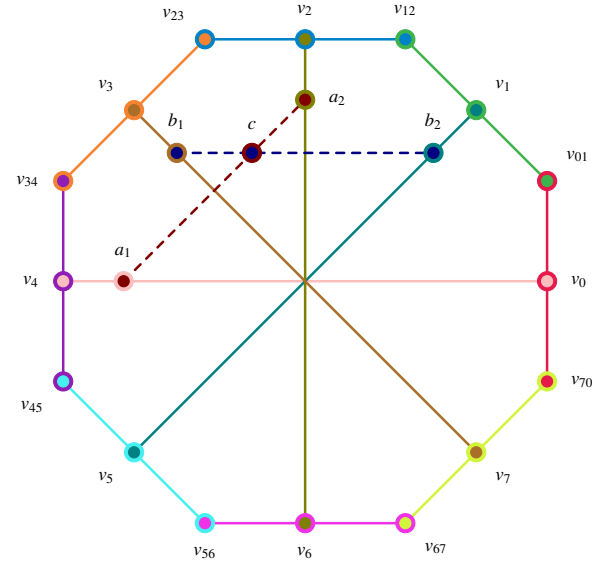
FIG. 3. Redraw of the octagon using exactly the same coordinates as Fig. 2(a)/(b). The 12 original contexts are drawn with solid lines in 12 distinct colors. The two additional C = 1 contexts are dashed and meet at the intertwining vertex c . Concentric disks mark vertices incident with two contexts.
