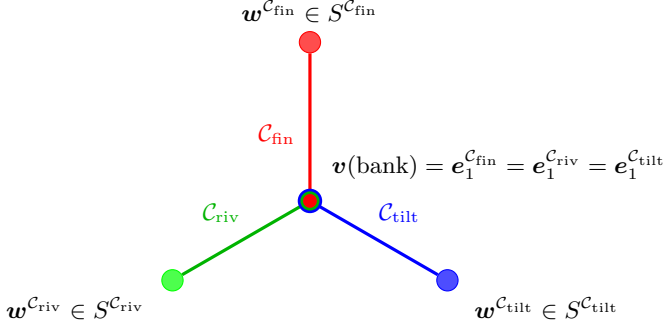
FIG. 1. Schematic of hinge-anchored frame sharing in the simplest single-link case. A candidate hinge vector associated with the token “bank” is shared by several possible sense frames. The colored outer nodes represent exemplary directions w^{c_{\text{fin}}} , w^{c_{\text{riv}}} , and w^{c_{\text{tilt}}} inside the corresponding sense subspaces, not the entire subspaces themselves. The formal model treats sense content as lying in low-dimensional subspaces of the hinge-perpendicular carrier v(\text{bank})^\perp . More generally, two contextual frames may share several link directions, in which case the relevant carrier is the orthogonal complement of the shared link subspace rather than of a single hinge vector.
