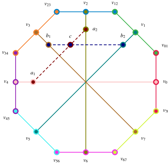
FIG. 3. Redraw of the octagon using exactly the same coordinates as Fig. 2(a)/(b). The 12 original contexts are drawn with solid lines in 12 distinct colors. The two additional C = 1 contexts are dashed and meet at the intertwining vertex c . Concentric disks mark vertices incident with two contexts.
