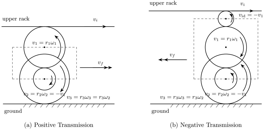
Figure 3: Schematic of the gearbox analogy in the laboratory frame G . The lower line represents the ground, which is stationary in this frame, and the arrow v_f denotes the speed of the gearbox/vehicle relative to the ground. Curved arrows indicate the sense of rotation, and the labels v_1 , v_2 , v_3 , and v_{id} denote local tangential speeds as defined in the text. The apparent sign mismatch at the upper rack–gear contact is resolved by the translation of the gearbox: because the gear center moves with the gearbox, the no-slip condition in the laboratory frame involves the absolute contact-point velocity, namely v_f - v_1 at the upper contact, not the tangential contribution -v_1 alone. (a) Positive transmission (downwind): the motion of the upper rack (wind) is transmitted through the gear train to the lower contact in the same sense, yielding velocity amplification. (b) Negative transmission (upwind): an idler gear reverses the transmitted sense of motion between the upper and lower contacts while preserving the same no-slip, ground-constrained coupling at the lower contact.
