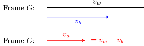
Figure 2: Minimal kinematic definitions for Sec. 4. In the laboratory frame G , the true wind is v_w and the boat speed is v_b . In the instantaneous boat frame C , the apparent-wind velocity is v_a = v_w - v_b . Vectors are aligned at a common origin; for v_b > v_w , the apparent-wind velocity v_a reverses direction.
