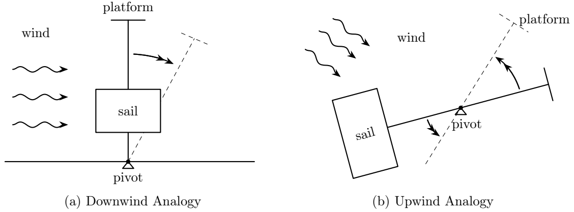
Figure 5: Schematic of the lever analogy. (a) For downwind motion, the pivot is at one end. The wind pushes the sail (at distance d_s ), causing the far end (at L ) to move faster than the wind. (b) For upwind motion, the pivot lies between the sail and the observation point, causing the far end to move in the opposite direction of the wind’s push.
