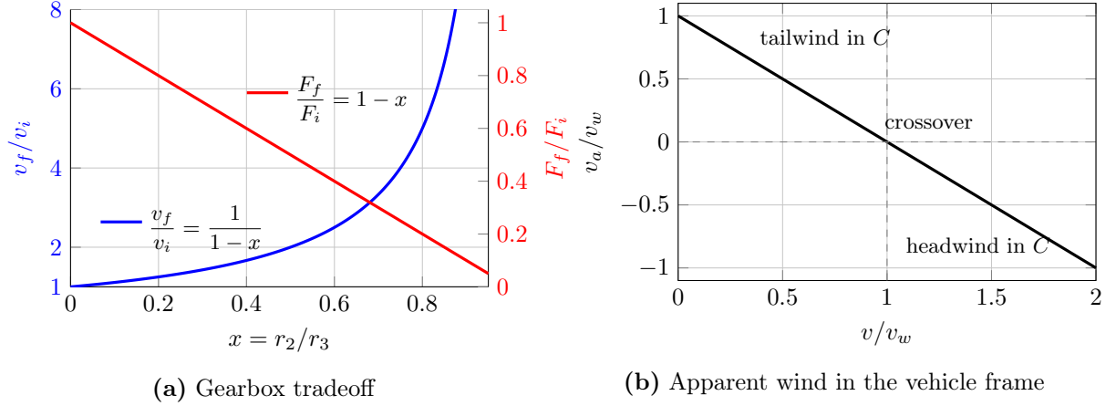
Figure 4: Dimensionless plots of two key relations used in the text. (a) In the gearbox analogy, with x = r_2/r_3 , the ideal speed amplification \frac{v_f}{v_i} = \frac{1}{1-x} increases as x \rightarrow 1^- , while the transmitted force ratio \frac{F_f}{F_i} = 1 - x decreases correspondingly. This illustrates the force-speed tradeoff of the lossless transmission. (b) In the vehicle frame C , the apparent wind satisfies \frac{v_a}{v_w} = 1 - \frac{v}{v_w} . It is positive for v < v_w , vanishes at the crossover v = v_w , and becomes negative for v > v_w , meaning that the air then approaches from ahead in the vehicle frame.
