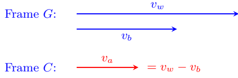
FIG. 2. Minimal kinematic definitions for Sec. IV. In the laboratory frame G , the true wind is v_w and the boat speed is v_b . In the instantaneous boat frame C , the apparent-wind velocity is v_a = v_w - v_b . Vectors are aligned at a common origin; for v_b > v_w , the apparent-wind velocity v_a reverses direction.
