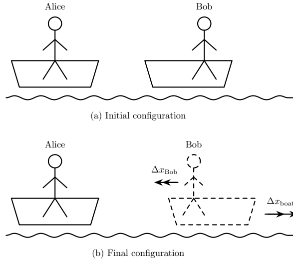
Figure 6: Schematic of the “Popescu Glide” thought experiment. (a) Initial configuration. (b) Final configuration after Bob attempts to move toward Alice: Bob moves leftward within his frictionless boat while the boat recoils rightward. Without an external interaction, such as paddling in the water, the center of mass of the Bob–boat system remains fixed, and he cannot achieve net propulsion.
