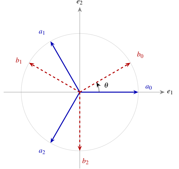
FIG. 1. The Mercedes-Benz pseudocontext of Example 19, drawn for \theta = \pi/6 . The solid blue rays a_0, a_1, a_2 and the dashed red rays b_0, b_1, b_2 are two distinct unordered triples in the plane V , yet the associated rank-one projectors have the same sum \frac{3}{2}I_V .
