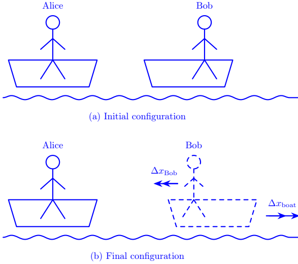
FIG. 6. Schematic of the “Popescu Glide” thought experiment. (a) Initial configuration. (b) Final configuration after Bob attempts to move toward Alice: Bob moves leftward within his frictionless boat while the boat recoils rightward. Without an external interaction, such as paddling in the water, the center of mass of the Bob–boat system remains fixed, and he cannot achieve net propulsion.
