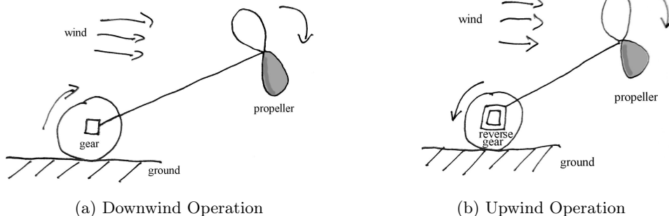
FIG. 1. Schematic of a wind-driven vehicle's operation. Arrows indicate the direction of rotation. The pitch of the propeller blades is indicated by the darker shade of the blade facing the rear. (a) For downwind travel faster than the wind, the wheels drive the propeller, which pushes air backward to generate thrust. (b) For upwind travel, the wind turns the propeller (acting as a turbine), which drives the wheels and pulls the vehicle against the wind.
