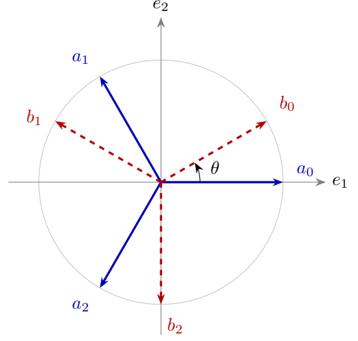
FIG. 1. A real size-three quantum pseudocontext, drawn for \theta = \pi/6 . The two triples are distinct tight frames with common structure operator (3/2)I_2 .
