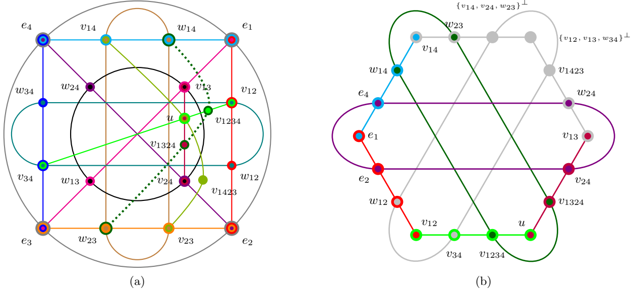
FIG. 2. (a) Four-dimensional extension of the Hardy–Salinas Schmeis hypergraph notation [15]. Solid curves show imposed contexts. The dotted dark-green curve is the equality-induced context \mathcal{E}_3 = \{w_{14}, w_{23}, v_{1234}, v_{1324}\} ; the other contexts of the complete 20-ray orthogonality hypergraph are listed in the text. (b) The Cabello 18-ray, 9-context KS configuration [10], with labels from Ref. [2]. Shared rays are relabeled by the gadget notation; overall nonzero scalar factors are immaterial. The notation \{v_i, v_j, v_k\}^\perp denotes the unique ray orthogonal to the span of three independent rays. The drawings record the stated incidence relations; no lattice-theoretic conclusion is inferred from the planar layout alone.
