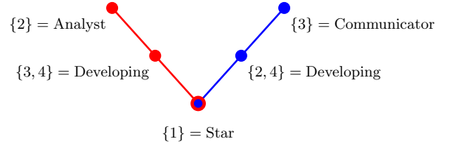
FIG. 1. Greechie orthogonality diagram (hypergraph) of the L_{12} personnel-assessment logic. Each line represents one context—one available mode of observation. The written-test context C_W (left) carries three observed categories: the singleton \{2\} (Analyst, recognizable by adequate test performance), the pair \{3, 4\} (Communicator and Developing, conflated because both score poorly on the analytical task), and the singleton \{1\} (Star, top scorer). The interview context C_I (right) carries a different triple of observed categories: \{3\} is now resolved (Communicator, identifiable by social poise) but \{2, 4\} is conflated (Analyst and Developing, both weak in interpersonal tasks). The observed category \{1\} is the intertwining atom : it appears in both contexts because the Star’s latent social profile—excellence on both dimensions—makes this profile identifiable regardless of which instrument is chosen. The five observed categories, together with their lattice-theoretic joins and meets, generate a 12-element non-Boolean logic, hence the name L_{12} .
