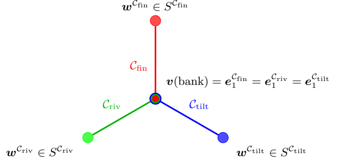
FIG. 2. Schematic of hinge-anchored frame sharing in the simplest single-link case. A candidate hinge vector associated with the token “bank” is shared by several possible sense frames. The colored outer nodes represent exemplary directions w^{C_{\text{fin}}} , w^{C_{\text{riv}}} , and w^{C_{\text{tilt}}} inside the corresponding sense subspaces, not the entire subspaces themselves. The formal model treats sense content as lying in low-dimensional subspaces of the hinge-perpendicular carrier v(\text{bank})^{\perp} . More generally, two contextual frames may share several link directions, in which case the relevant carrier is the orthogonal complement of the shared link subspace rather than of a single hinge vector.
