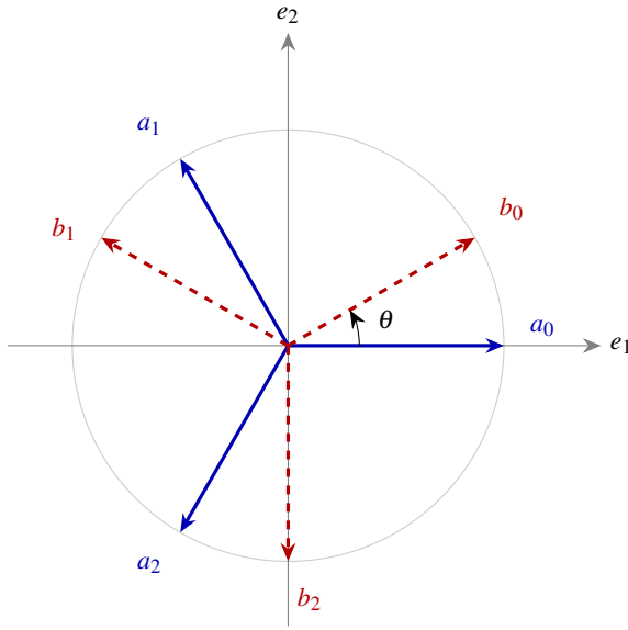
FIG. 1. The Mercedes–Benz pseudocontext of Example 19, drawn for \theta = \pi/6 . The solid blue rays a_0, a_1, a_2 and the dashed red rays b_0, b_1, b_2 are two distinct unordered triples in the plane V , yet the associated rank-one projectors have the same sum \frac{3}{2}I_V .
