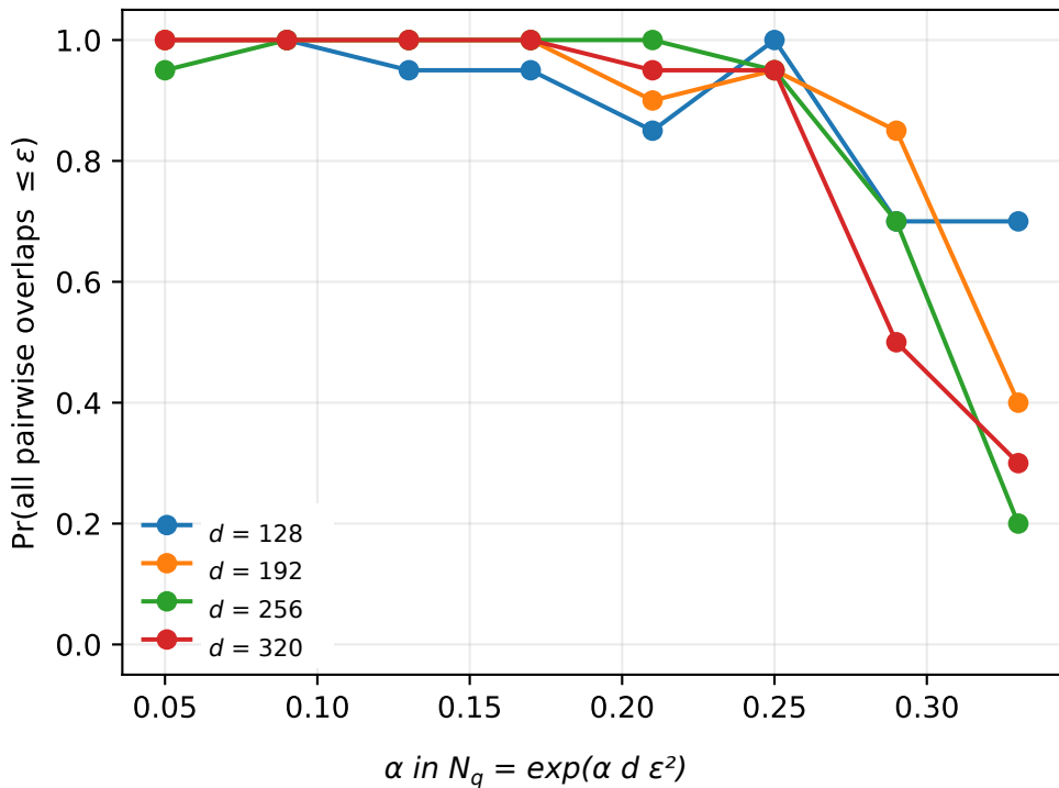
Quasi-orthogonal coexistence, \varepsilon = 0.25
