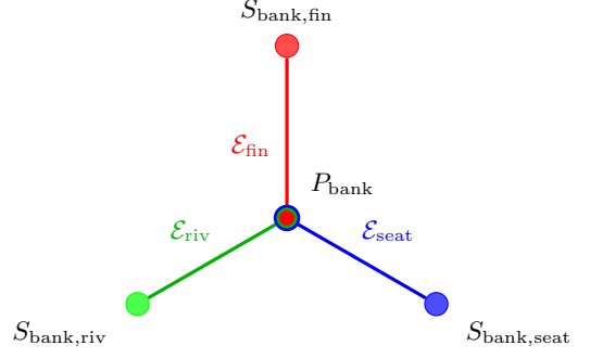
FIG. 1. Structural incidence schematic for the lexically ambiguous token “bank.” The center is the shared lexical projector P_{\text{bank}} ; the outer nodes represent displayed residual sectors for the financial, river-edge, and seat/bench contexts. Each colored arm is only the visible fragment of a context hyperedge; omitted mutually orthogonal vertices complete its basis. When m_s > 1 , an outer S_{t,s} node compresses several rank-one projector vertices associated with an orthonormal basis of that residual subspace; it is not itself one rank-one quantum outcome. The concentric colors mark membership of the same projector in all three contexts. The diagram records shared incidence only, not a vector, map, causal arrow, Born-rule measurement, or claim about what an existing Transformer has learned.
