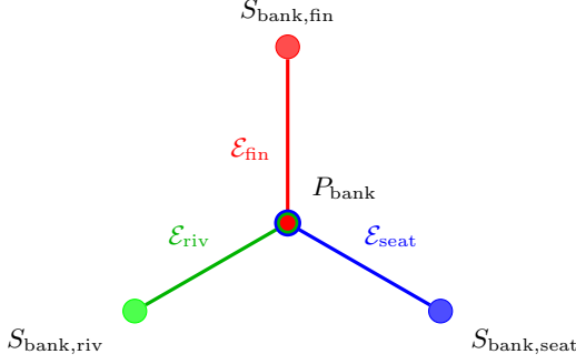
FIG. 1. Structural incidence schematic for the lexically ambiguous token “bank.” The center is the shared lexical projector P_{\text{bank}} ; the outer nodes represent displayed residual sectors for the financial, river-edge, and seat/bench contexts. Each colored arm is only the visible fragment of a context hyperedge; omitted mutually orthogonal vertices complete its basis. When m_s > 1 , an outer S_{t,s} node compresses several rank-one projector vertices associated with an orthonormal basis of that residual subspace; it is not itself one rank-one quantum outcome. The concentric colors mark membership of the same projector in all three contexts. The diagram records shared incidence only, not a vector, map, causal arrow, Born-rule measurement, or claim about what an existing Transformer has learned.
