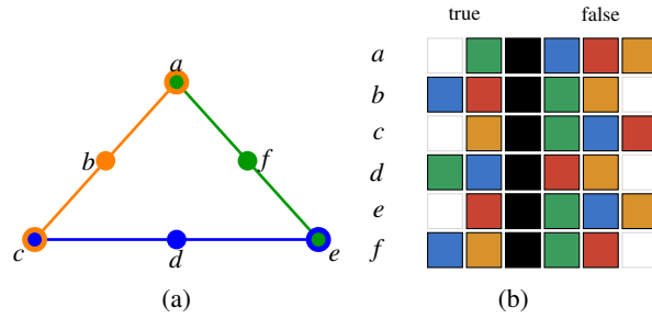
FIG. 3. A triangle-logic generalization of the Quantum Square . (a) Greechie-style depiction of the triangle logic associated with Eq. (28). The intertwining atoms a , c , and e are shown by concentric circles because each belongs to two contexts. (b) A tile rendering obtained from the grammar in Eq. (33), using four recurring state colors and a black separator between support and complement.
