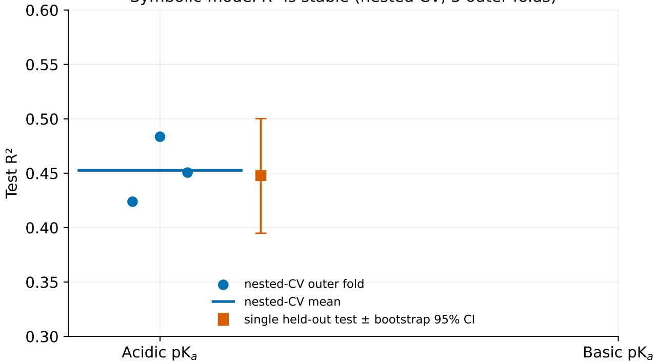
Symbolic-model R^2 is stable (nested CV, 3 outer folds)
