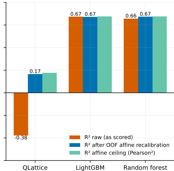
Basic pK_a — pooled external
