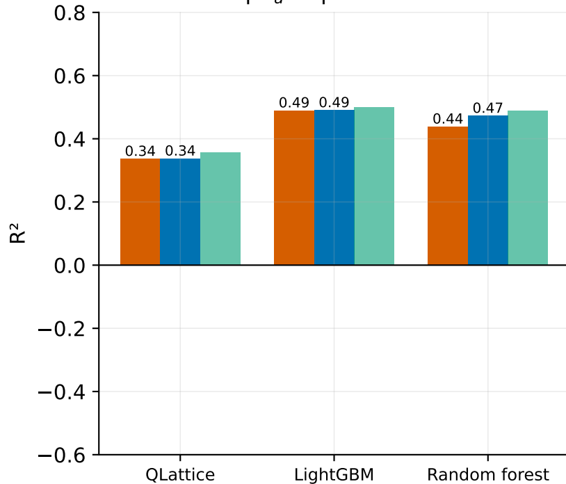
Acidic pK_a — pooled external
