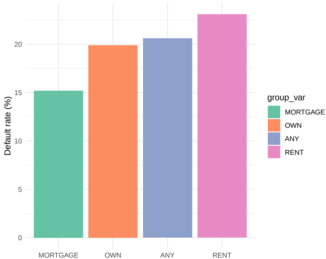
Default rate by group
