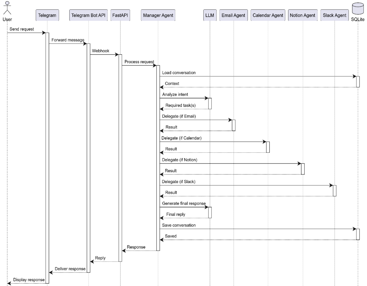
Synapse - Sequence Diagram
